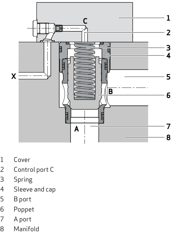
Directional Cartridge Valve and Cover
